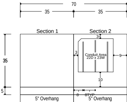
Front Plan View
