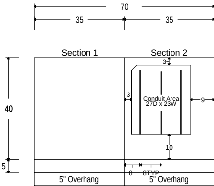
Front Plan View
