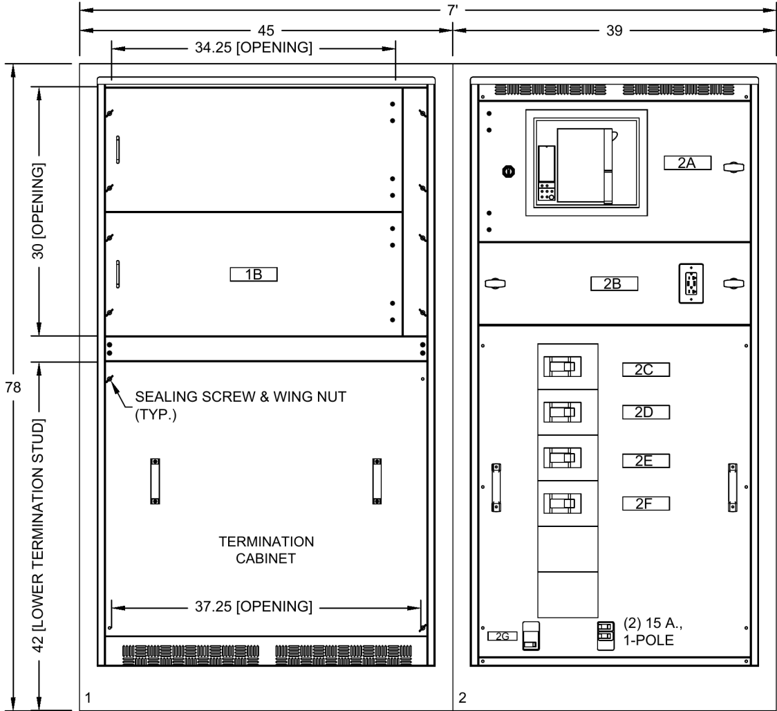
FRONT VIEW (SHOWN WITHOUT DOORS)
