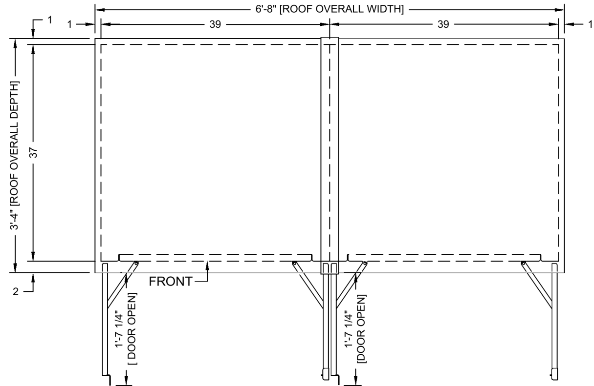
PLAN VIEW DOORS OPEN
