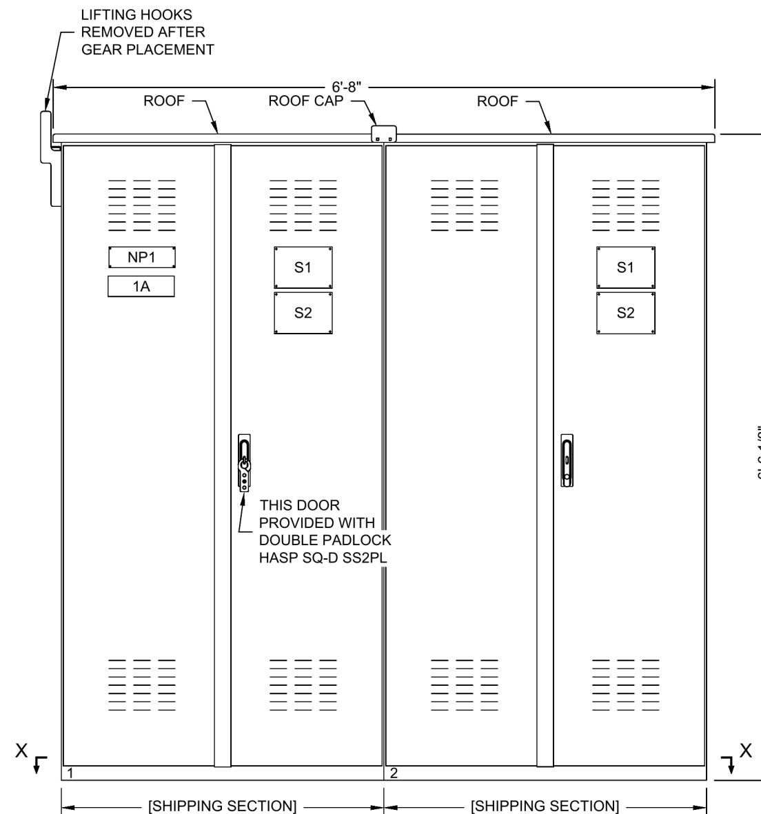
FRONT VIEW (EXTERIOR DOORS SHOWN)
