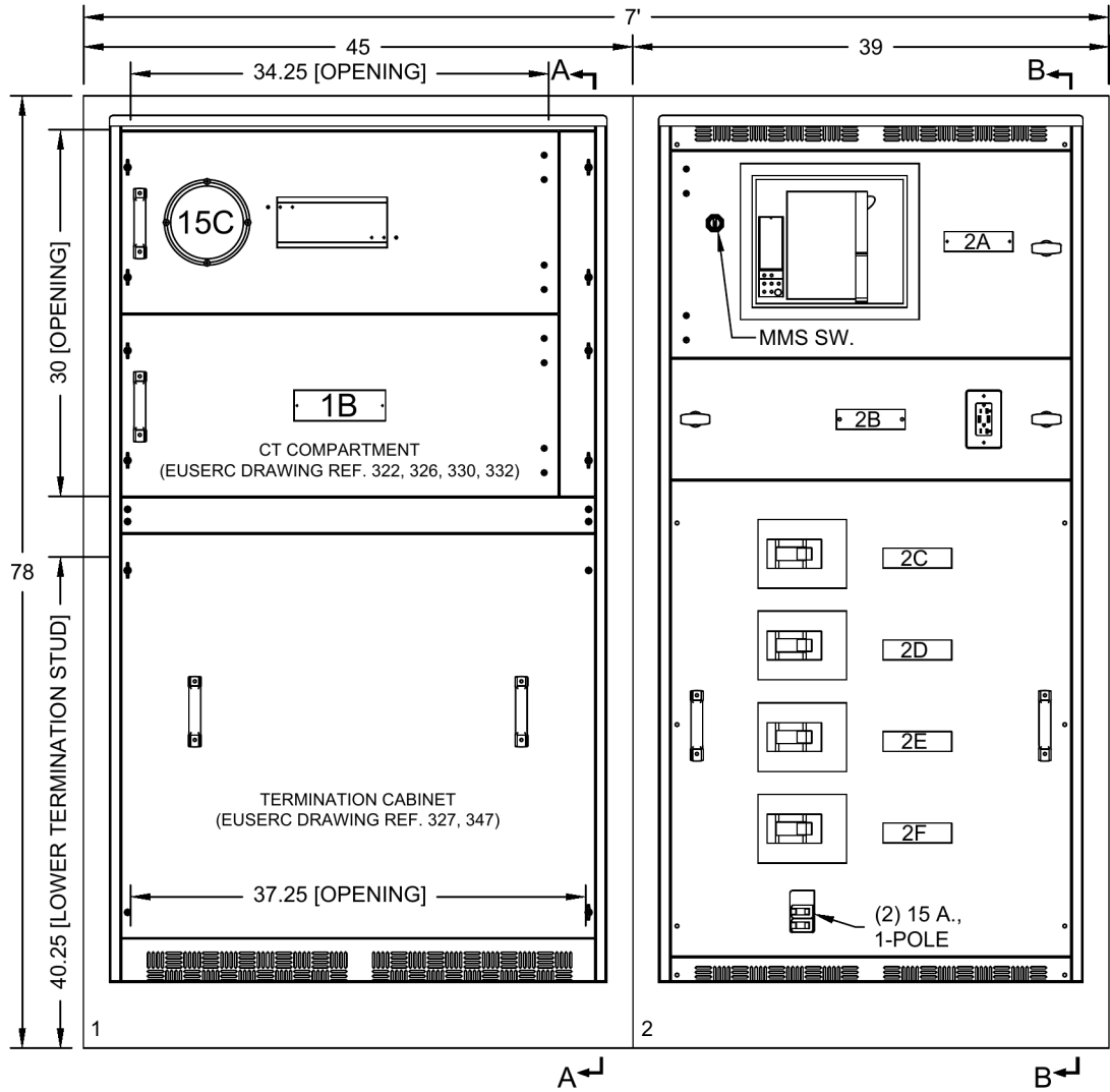
FRONT VIEW (SHOWN WITHOUT DOORS)
