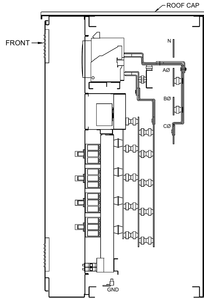
SECTION B-B
